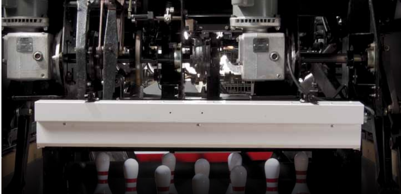
The 90XLi stores 20 pins and is always ready to spot a new set of pins.
